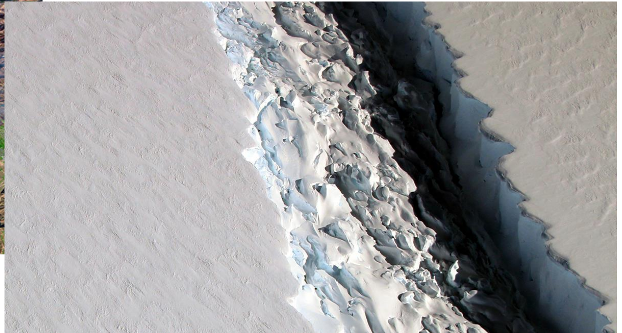
Larsen-C Ice Shelf; Image Credit: JPL SBG
